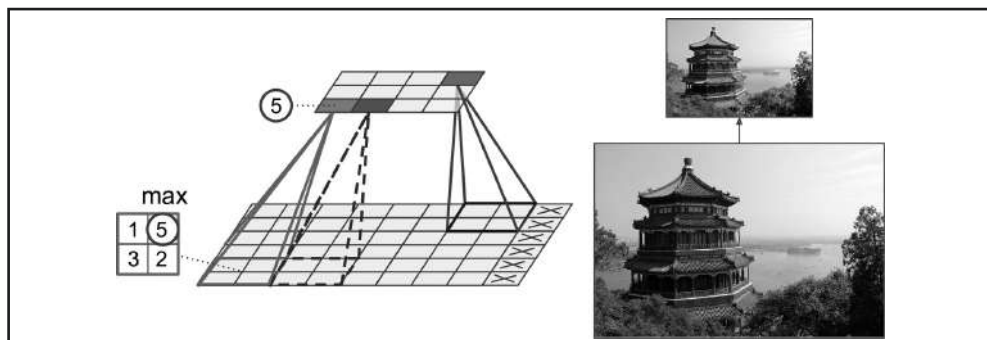
Figura 13-8. Camada max pooling (kernel pooling 2 \times 2 , stride de 2, sem padding)
