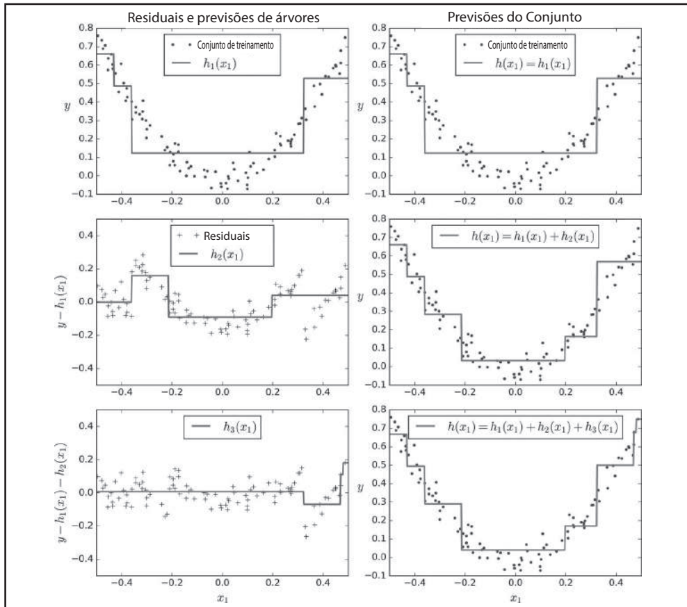
Figura 7-9. Gradient Boosting
