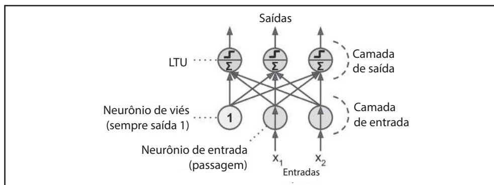
Figura 10-5. Diagrama Perceptron
