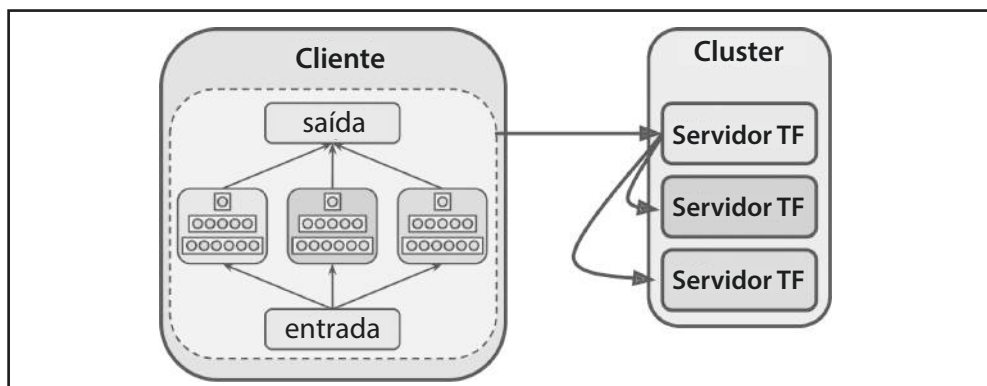
Figura 12-12. In-graph replication
