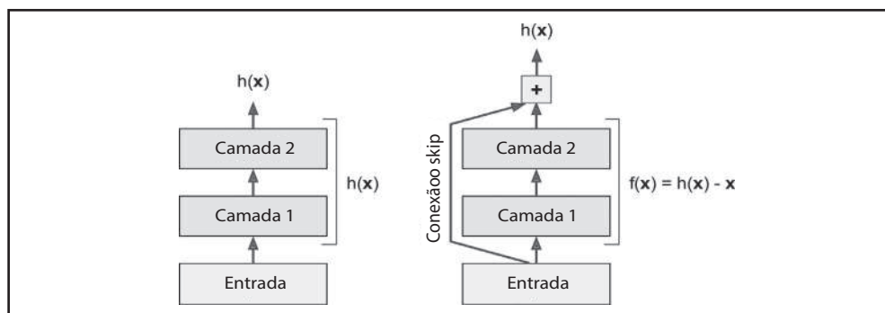
Figura 13-12. Residual Learning
